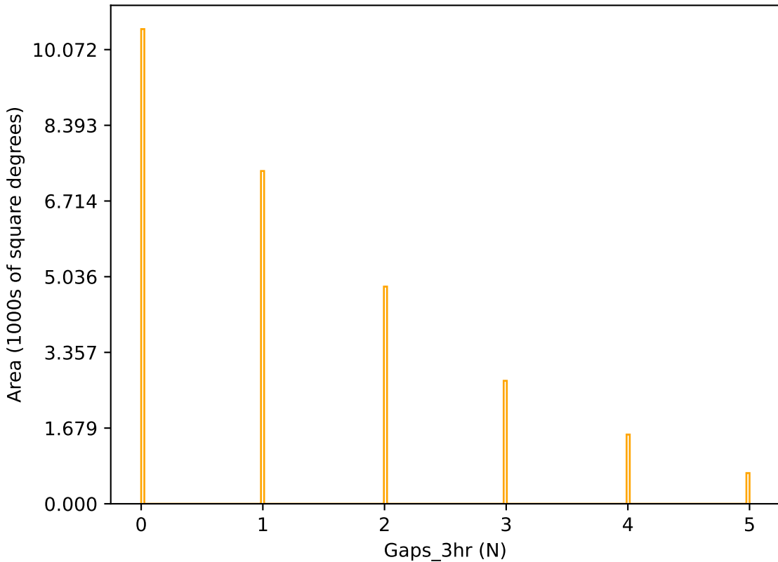
too_elab_r32_d3_ugrizy_v3.4_10yrs r band: Gaps_3hr
