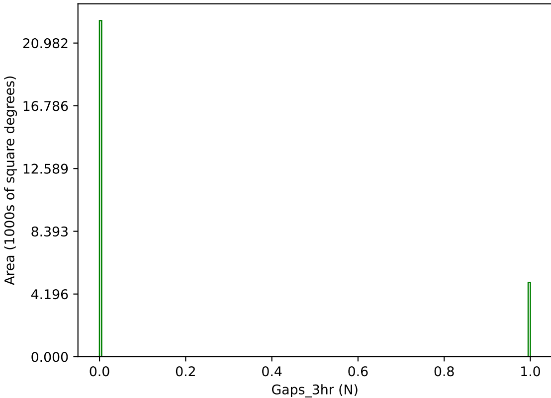
too_elab_r32_d3_ugrizy_v3.4_10yrs g band: Gaps_3hr
