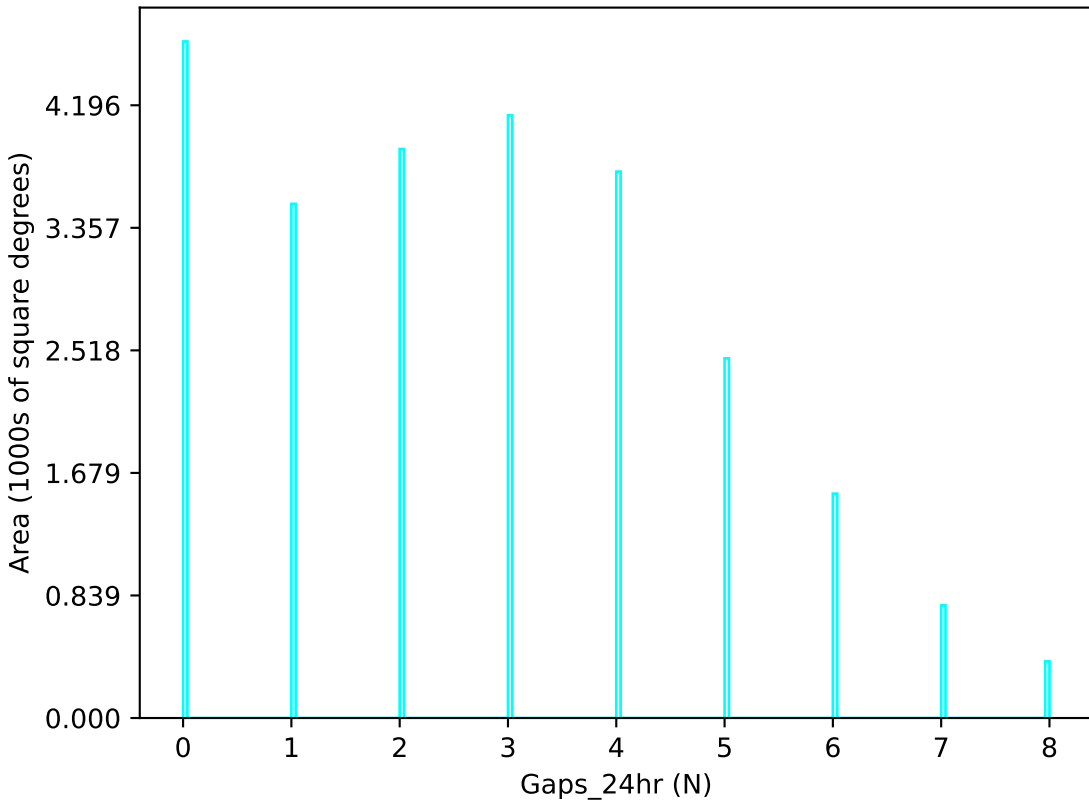
too_elab_r32_d3_ugrizy_v3.4_10yrs u band: Gaps_24hr
