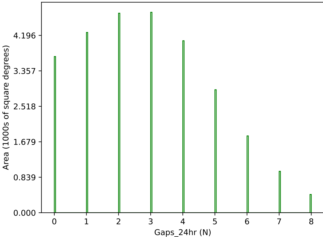
too_elab_r32_d3_ugrizy_v3.4_10yrs g band: Gaps_24hr
