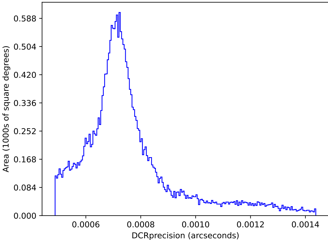
too_elab_r32_d3_ugrizy_v3.4_10yrs : DCRprecision
