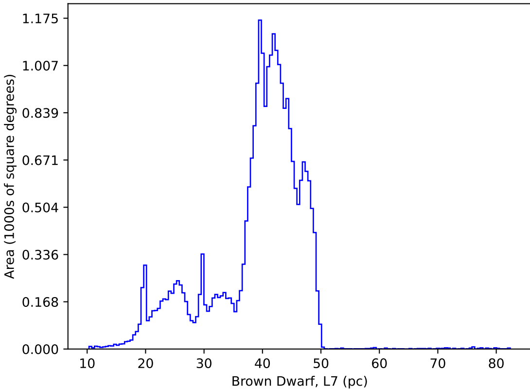
too_elab_r32_d3_ugrizy_v3.4_10yrs : Brown Dwarf, L7
