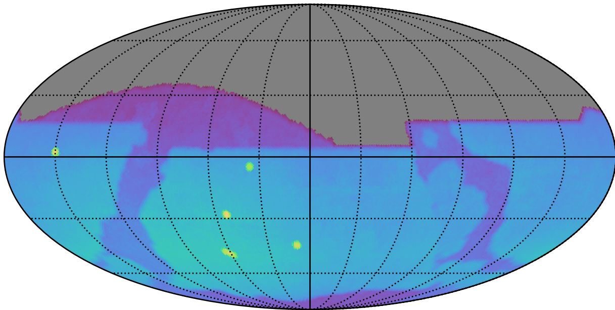
too_elab_r32_d3_ugrizy_v3.4_10yrs : Brown Dwarf, L4
