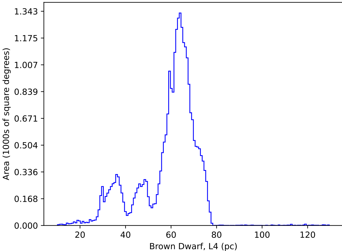
too_elab_r32_d3_ugrizy_v3.4_10yrs : Brown Dwarf, L4
