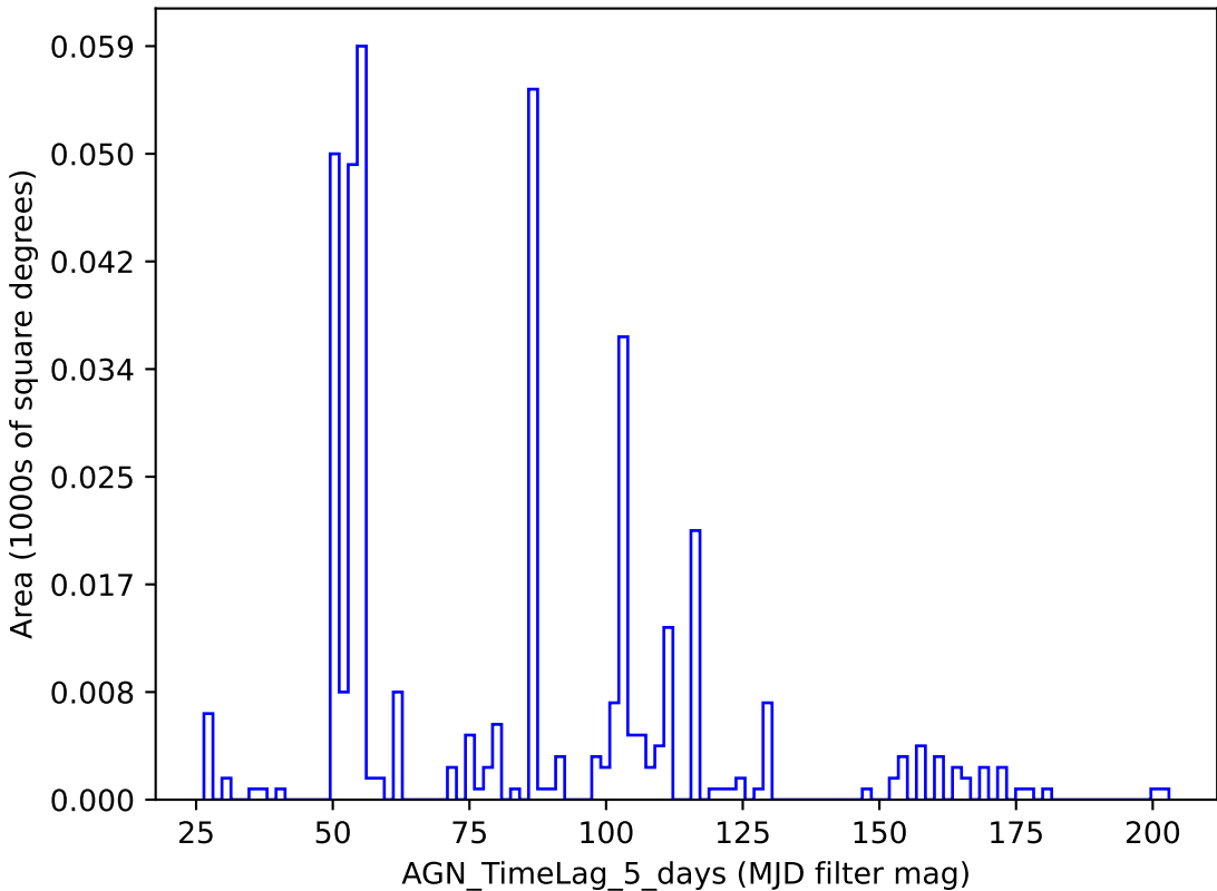
too_elab_r32_d3_ugrizy_v3.4_10yrs y band: AGN_TimeLag_5_days
