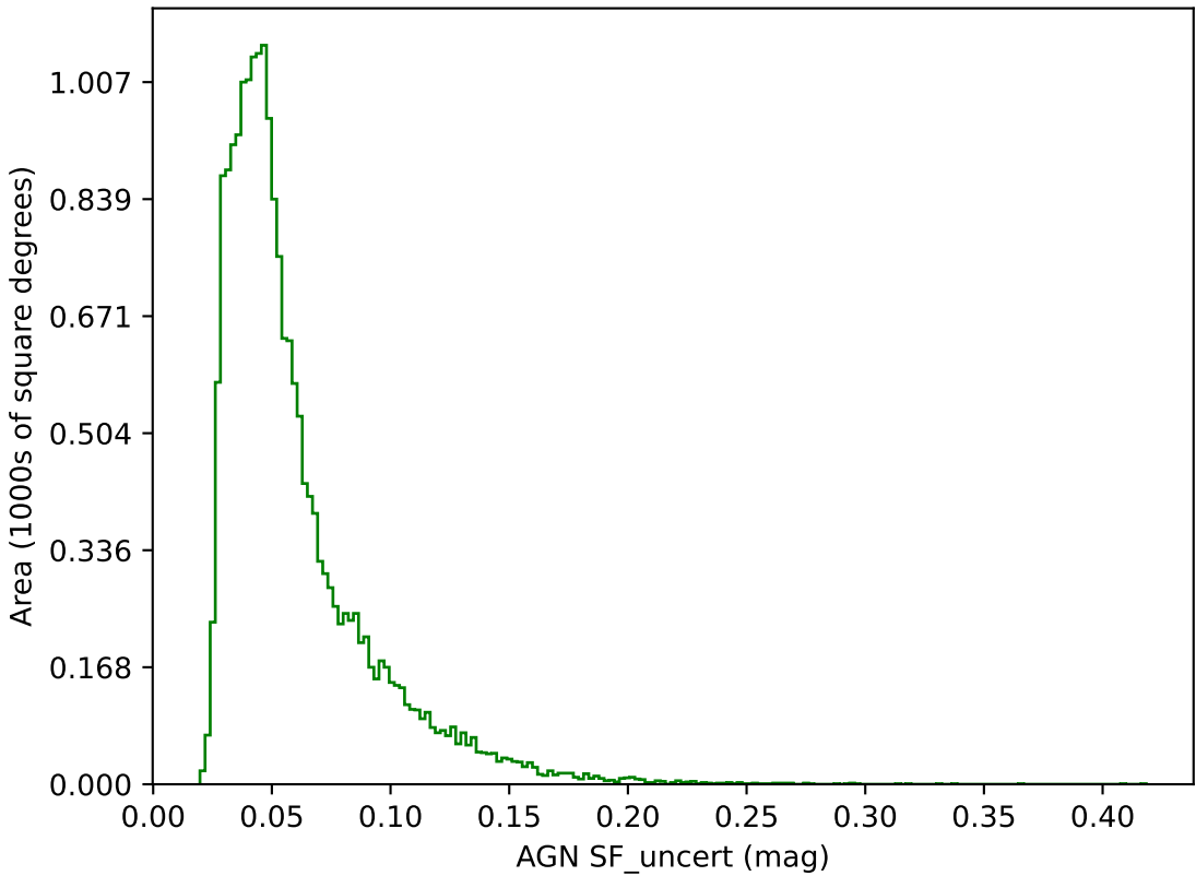
too_elab_r32_d3_ugrizy_v3.4_10yrs g band: AGN SF_uncert
