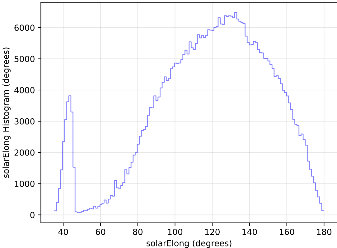
too_elab_r32_d3_ugrizy_v3.4_10yrs WFD z band: solarElong Histogram
