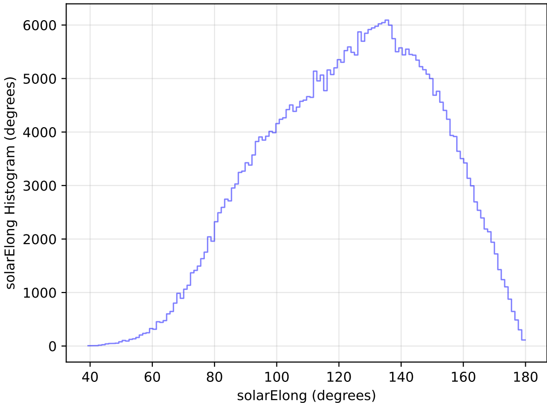
too_elab_r32_d3_ugrizy_v3.4_10yrs WFD y band: solarElong Histogram
