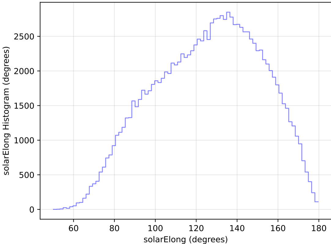
too_elab_r32_d3_ugrizy_v3.4_10yrs WFD u band: solarElong Histogram
