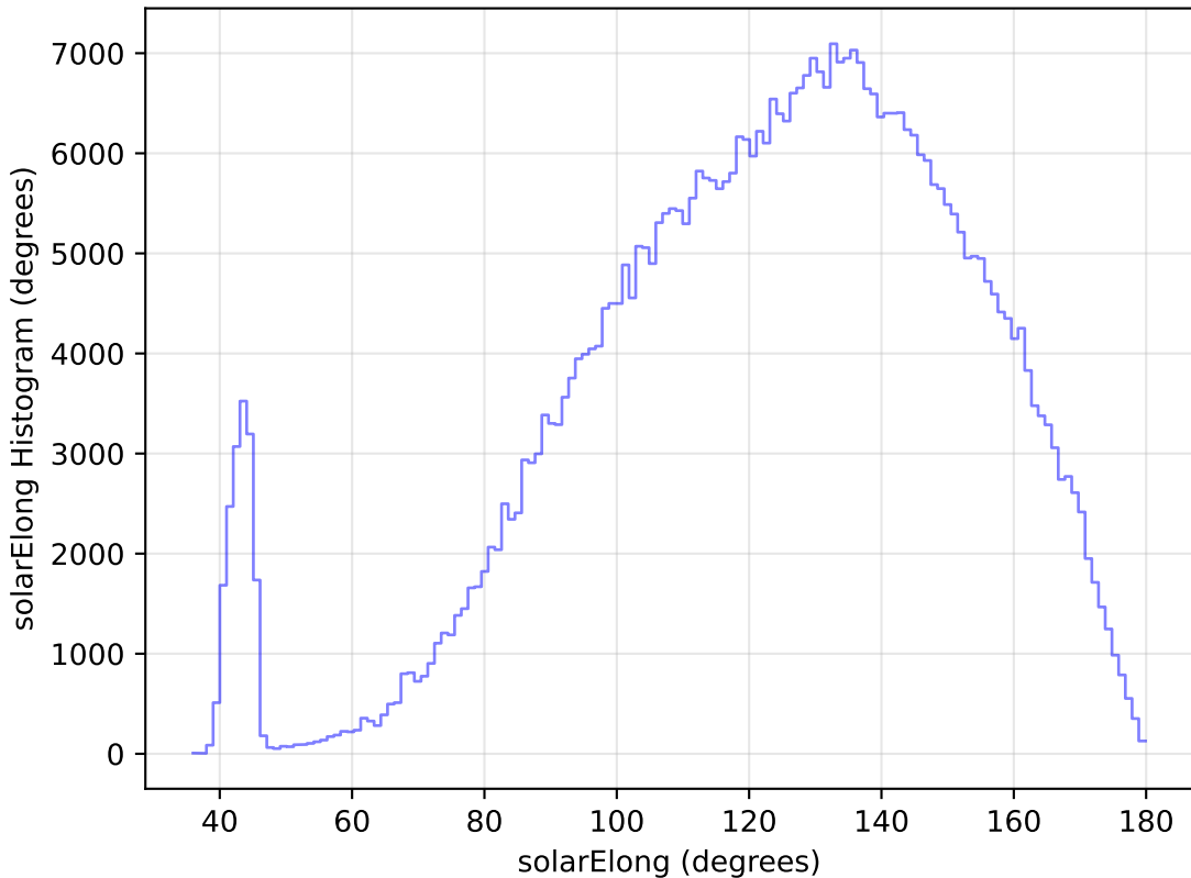
too_elab_r32_d3_ugrizy_v3.4_10yrs WFD r band: solarElong Histogram
