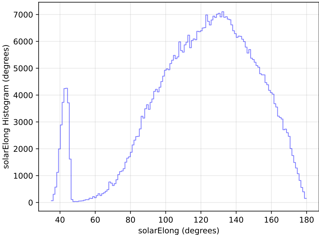
too_elab_r32_d3_ugrizy_v3.4_10yrs WFD i band: solarElong Histogram
