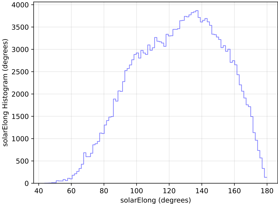
too_elab_r32_d3_ugrizy_v3.4_10yrs WFD g band: solarElong Histogram
