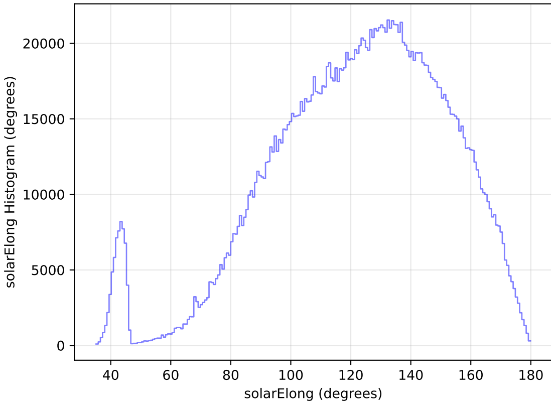
too_elab_r32_d3_ugrizy_v3.4_10yrs WFD all bands: solarElong Histogram
