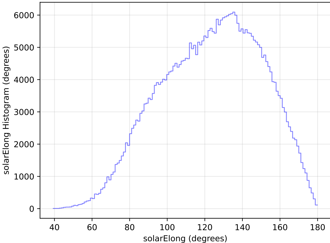
too_elab_r32_d3_ugrizy_v3.4_10yrs All sky y band: solarElong Histogram
