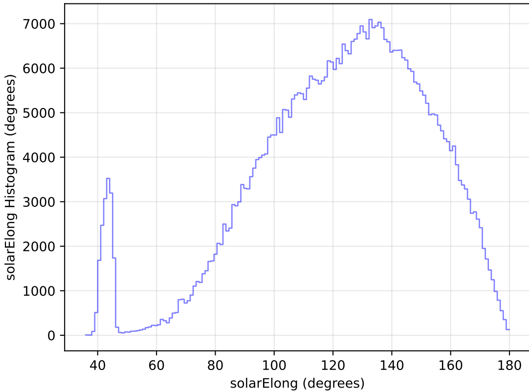
too_elab_r32_d3_ugrizy_v3.4_10yrs All sky r band: solarElong Histogram
