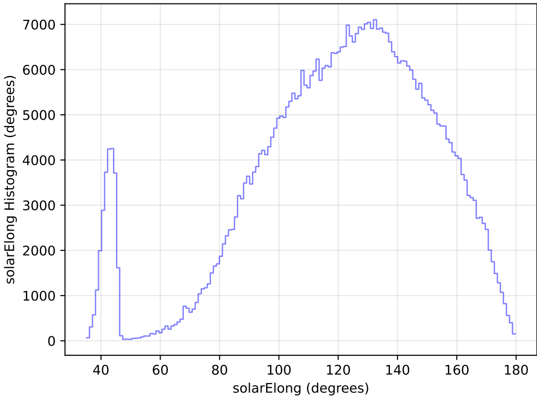
too_elab_r32_d3_ugrizy_v3.4_10yrs All sky i band: solarElong Histogram
