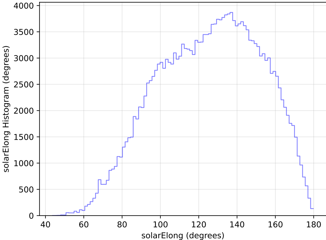
too_elab_r32_d3_ugrizy_v3.4_10yrs All sky g band: solarElong Histogram
