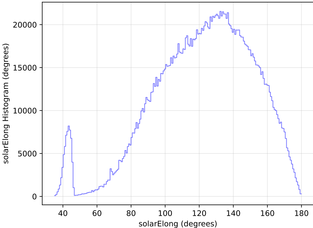
too_elab_r32_d3_ugrizy_v3.4_10yrs All sky all bands: solarElong Histogram
