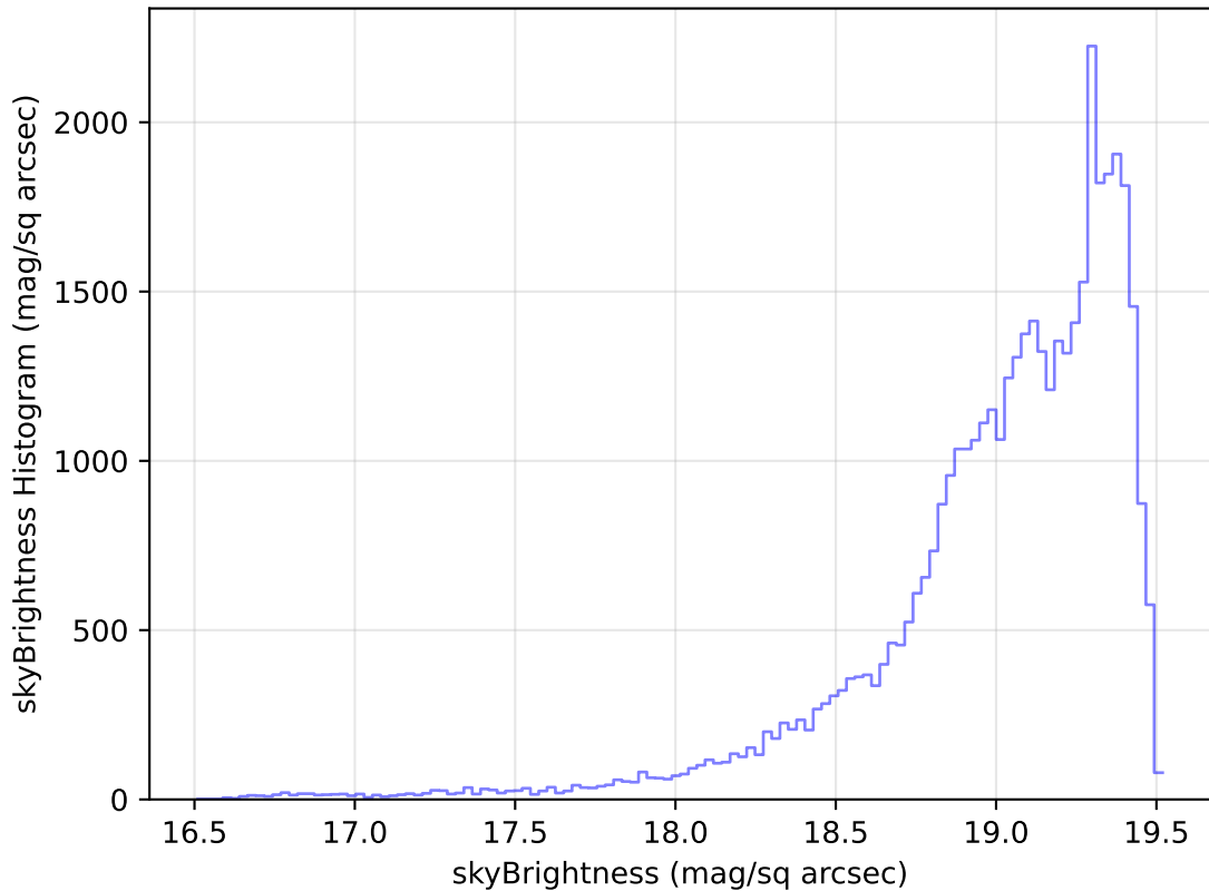
too_elab_r32_d3_ugrizy_v3.4_10yrs Yr 1 z band: skyBrightness Histogram
