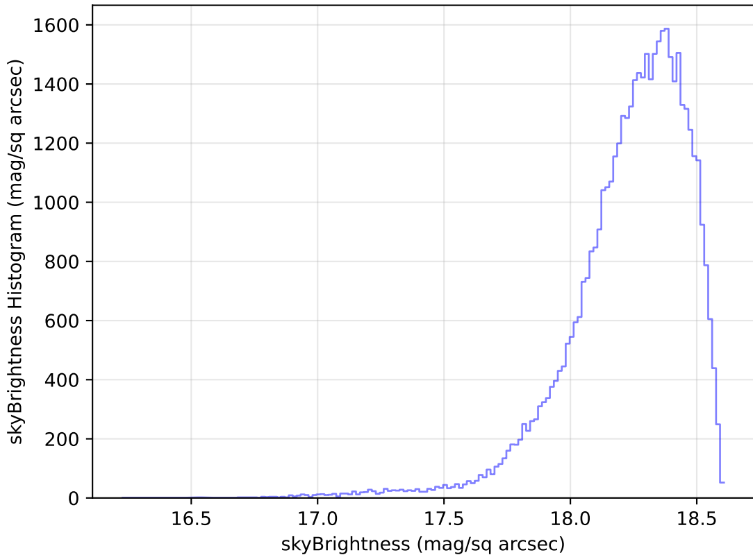
too_elab_r32_d3_ugrizy_v3.4_10yrs Yr 1 y band: skyBrightness Histogram
