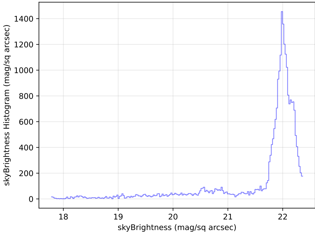
too_elab_r32_d3_ugrizy_v3.4_10yrs Yr 1 g band: skyBrightness Histogram
