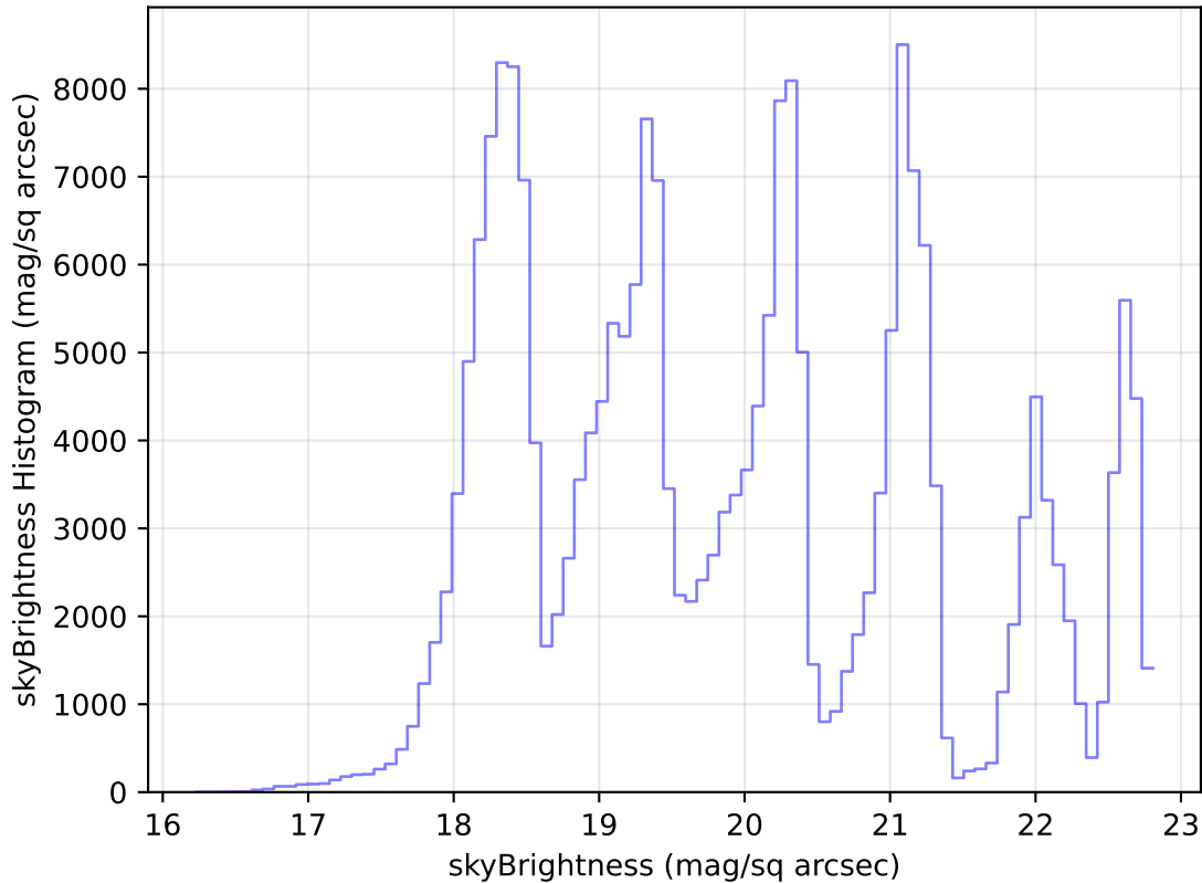
too_elab_r32_d3_ugrizy_v3.4_10yrs Yr 1 all bands: skyBrightness Histogram
