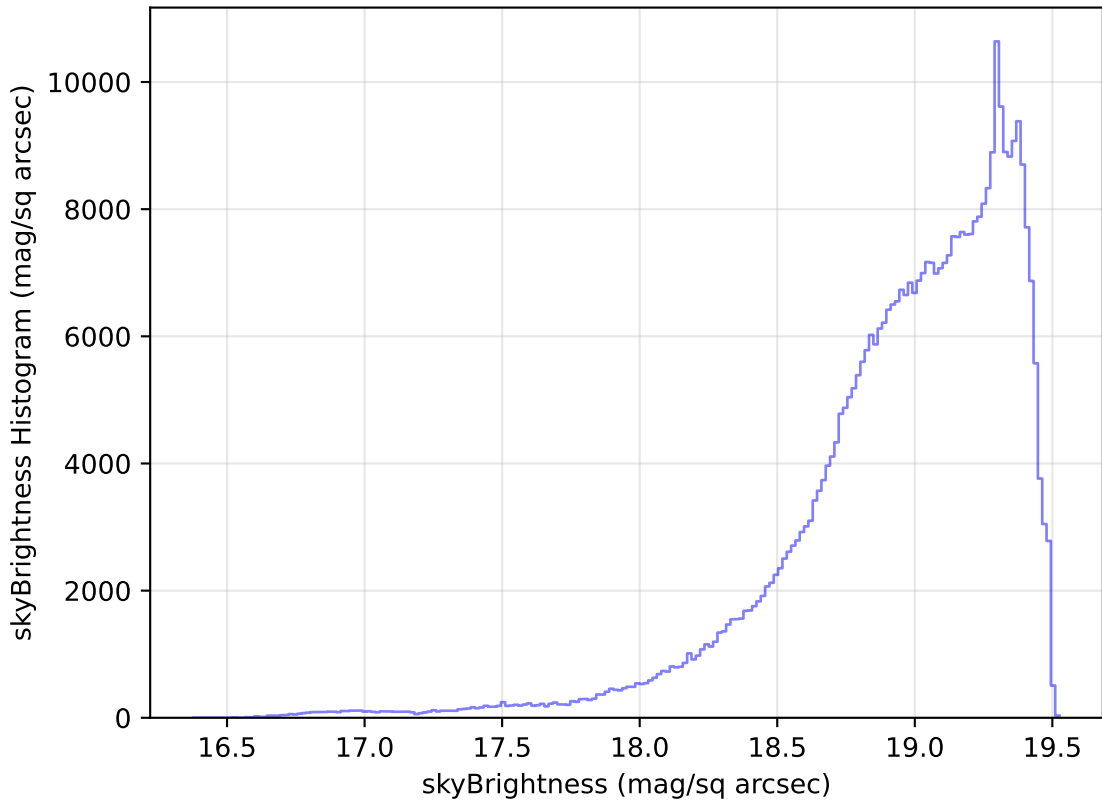
too_elab_r32_d3_ugrizy_v3.4_10yrs WFD z band: skyBrightness Histogram
