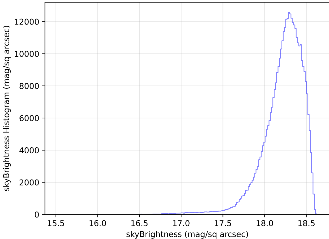
too_elab_r32_d3_ugrizy_v3.4_10yrs WFD y band: skyBrightness Histogram
