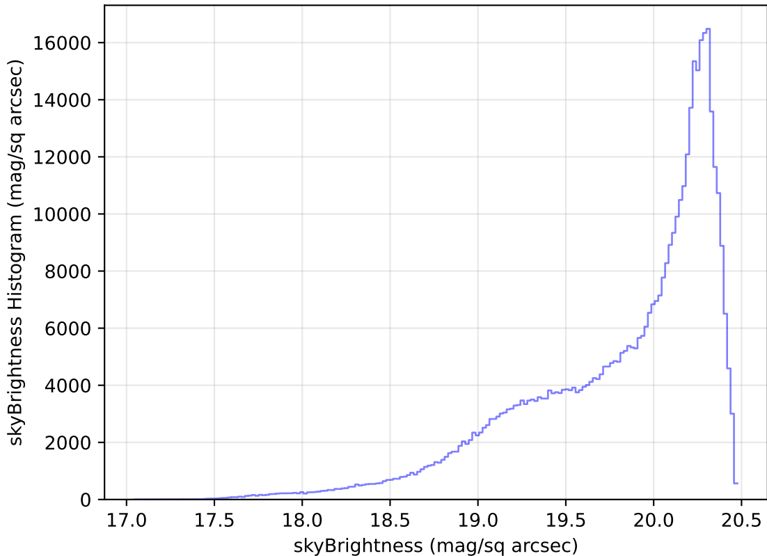
too_elab_r32_d3_ugrizy_v3.4_10yrs WFD i band: skyBrightness Histogram
