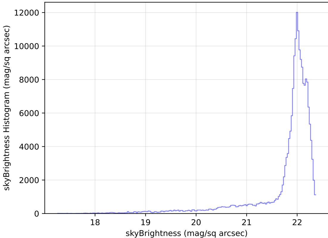
too_elab_r32_d3_ugrizy_v3.4_10yrs WFD g band: skyBrightness Histogram
