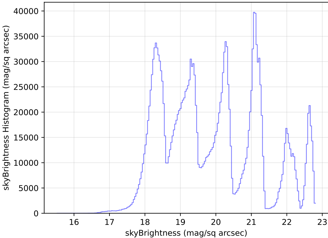
too_elab_r32_d3_ugrizy_v3.4_10yrs WFD all bands: skyBrightness Histogram
