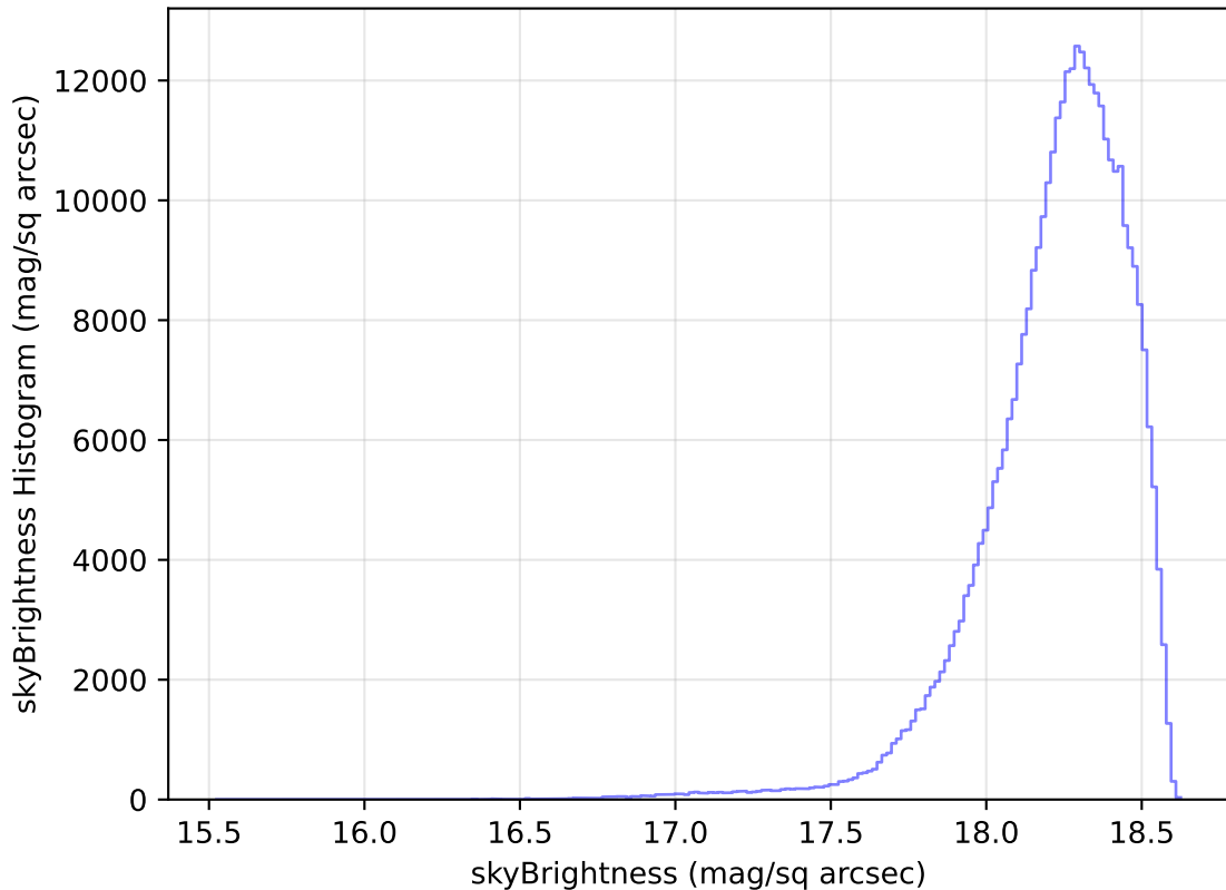
too_elab_r32_d3_ugrizy_v3.4_10yrs All sky y band: skyBrightness Histogram
