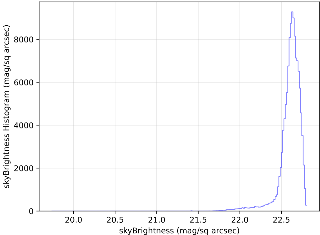
too_elab_r32_d3_ugrizy_v3.4_10yrs All sky u band: skyBrightness Histogram
