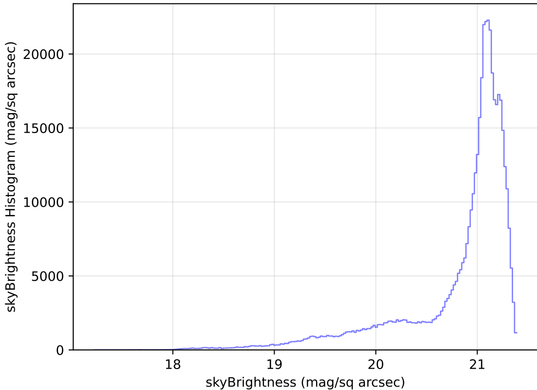
too_elab_r32_d3_ugrizy_v3.4_10yrs All sky r band: skyBrightness Histogram
