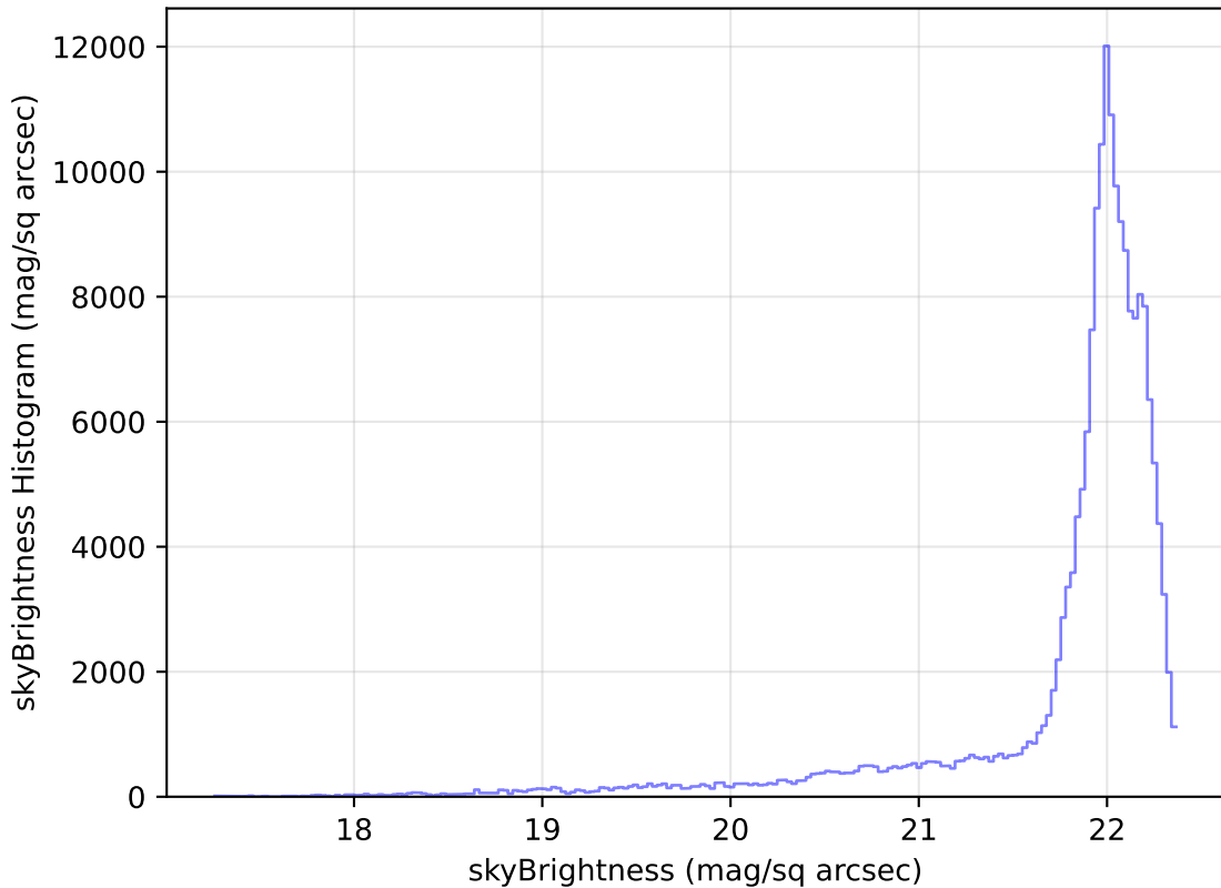
too_elab_r32_d3_ugrizy_v3.4_10yrs All sky g band: skyBrightness Histogram
