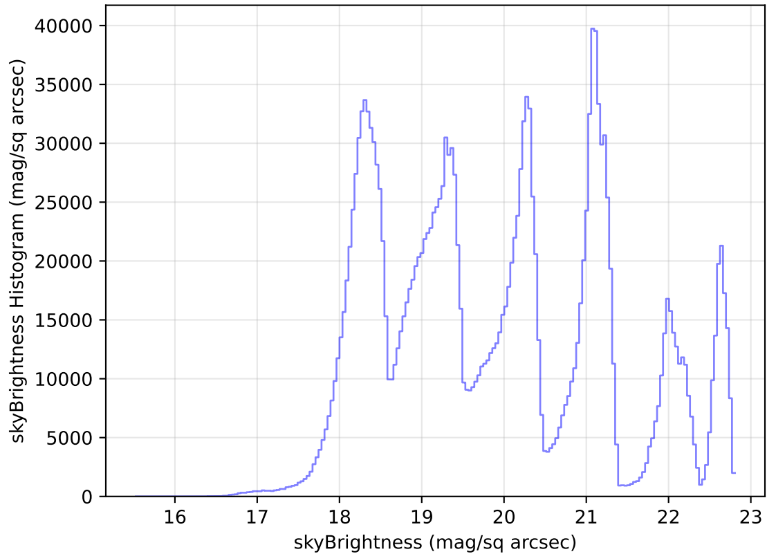
too_elab_r32_d3_ugrizy_v3.4_10yrs All sky all bands: skyBrightness Histogram
