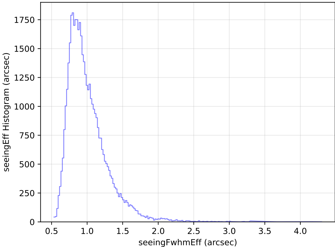
too_elab_r32_d3_ugrizy_v3.4_10yrs Yr 1 z band: seeingEff Histogram
