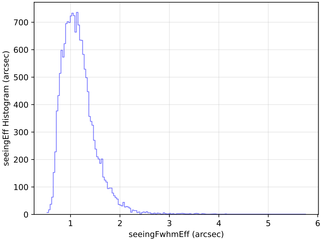
too_elab_r32_d3_ugrizy_v3.4_10yrs Yr 1 u band: seeingEff Histogram
