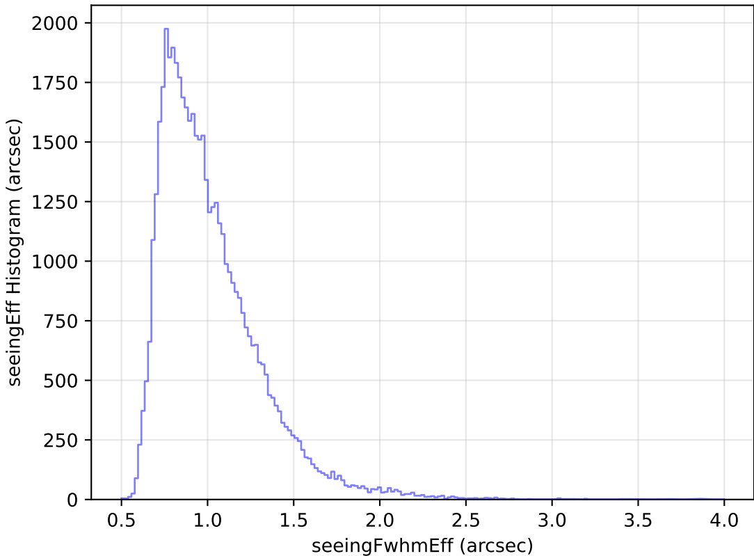
too_elab_r32_d3_ugrizy_v3.4_10yrs Yr 1 r band: seeingEff Histogram
