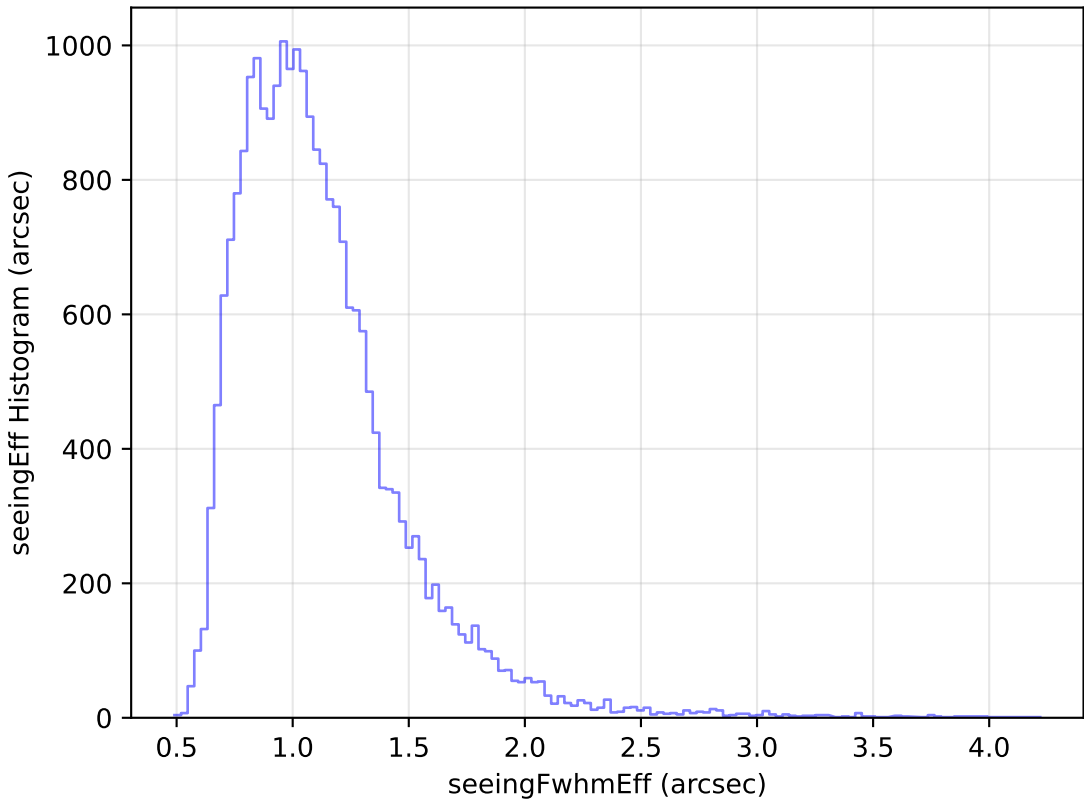
too_elab_r32_d3_ugrizy_v3.4_10yrs Yr 1 g band: seeingEff Histogram
