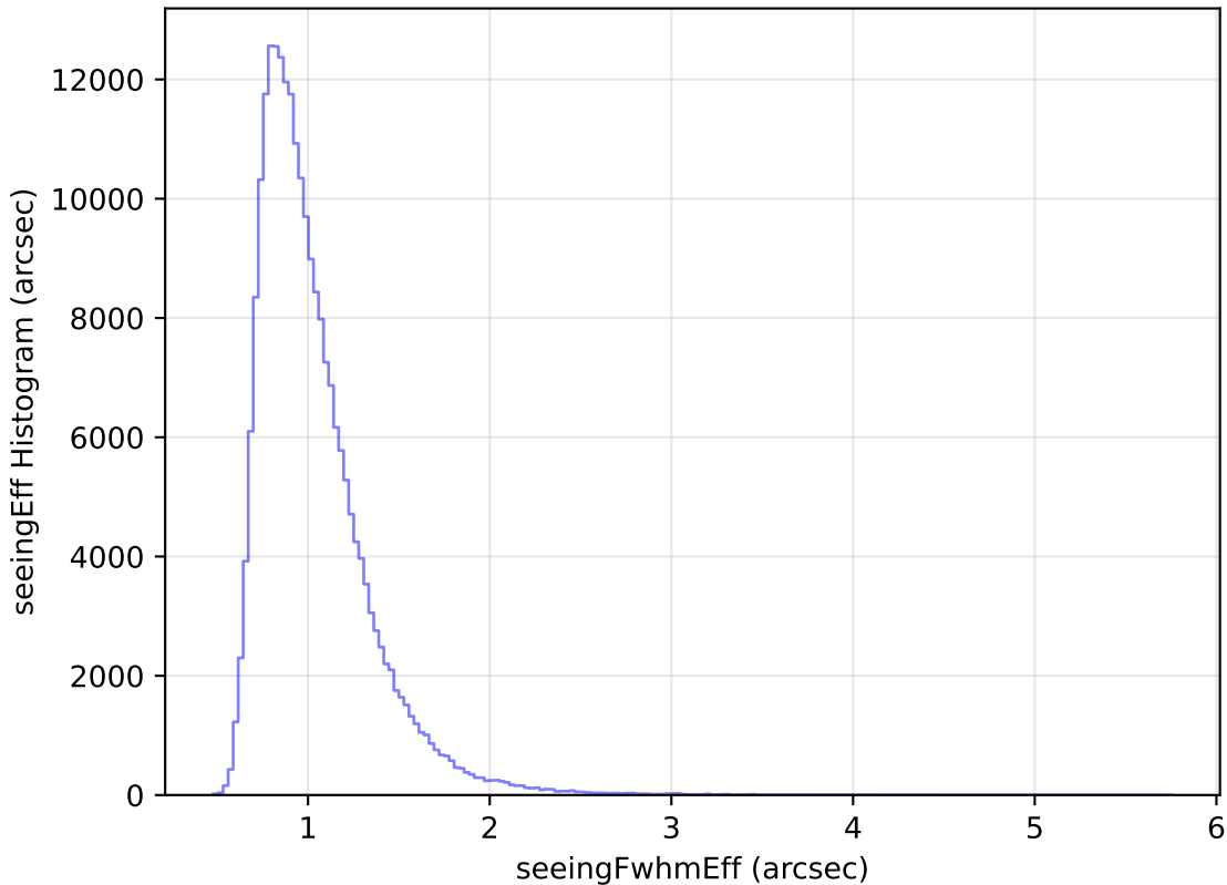
too_elab_r32_d3_ugrizy_v3.4_10yrs Yr 1 all bands: seeingEff Histogram
