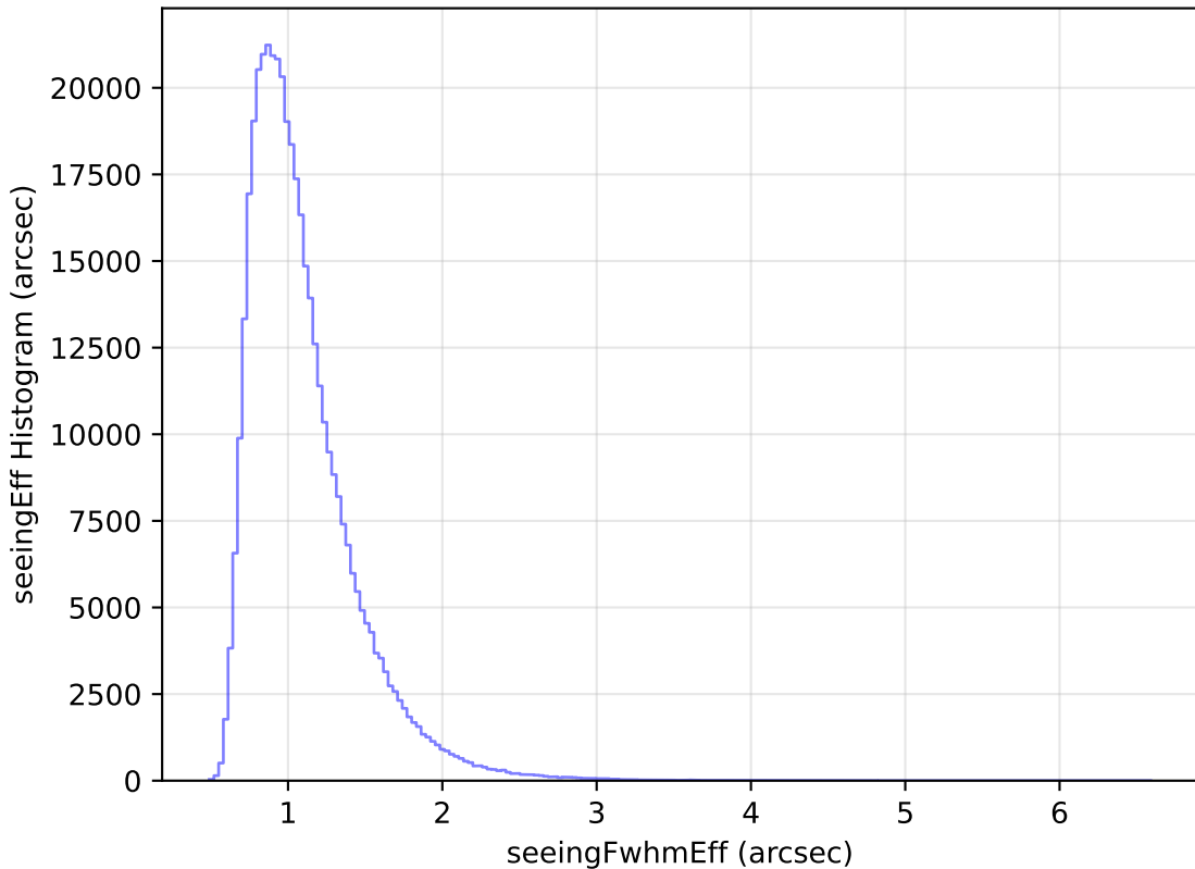
too_elab_r32_d3_ugrizy_v3.4_10yrs WFD z band: seeingEff Histogram
