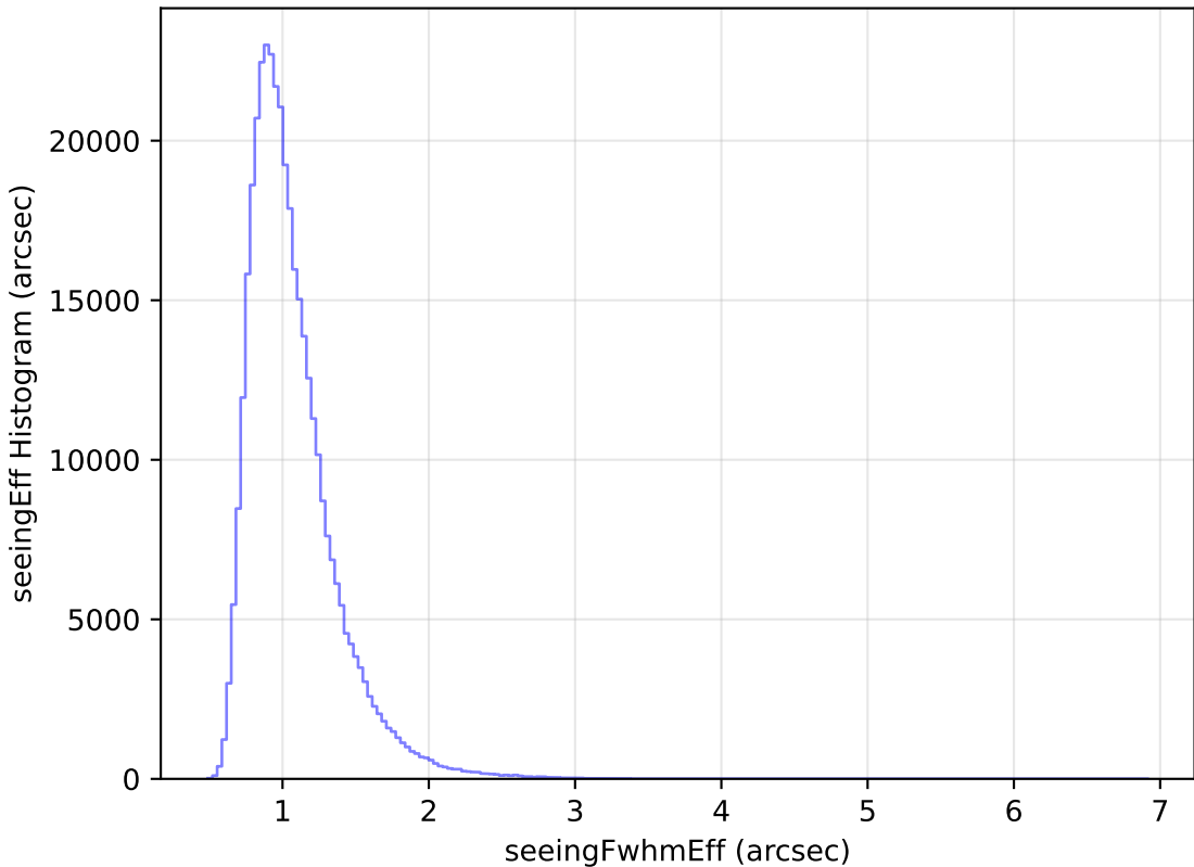
too_elab_r32_d3_ugrizy_v3.4_10yrs WFD y band: seeingEff Histogram
