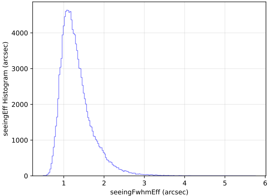
too_elab_r32_d3_ugrizy_v3.4_10yrs WFD u band: seeingEff Histogram
