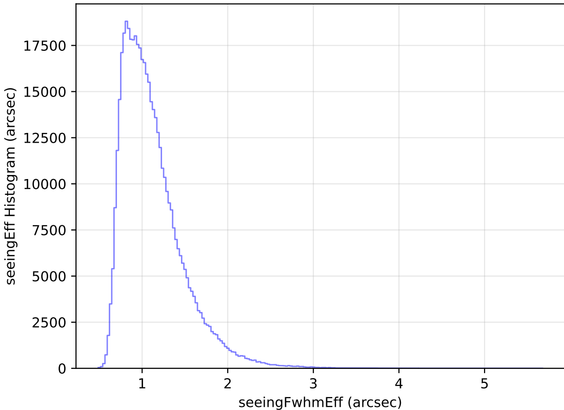
too_elab_r32_d3_ugrizy_v3.4_10yrs WFD r band: seeingEff Histogram
