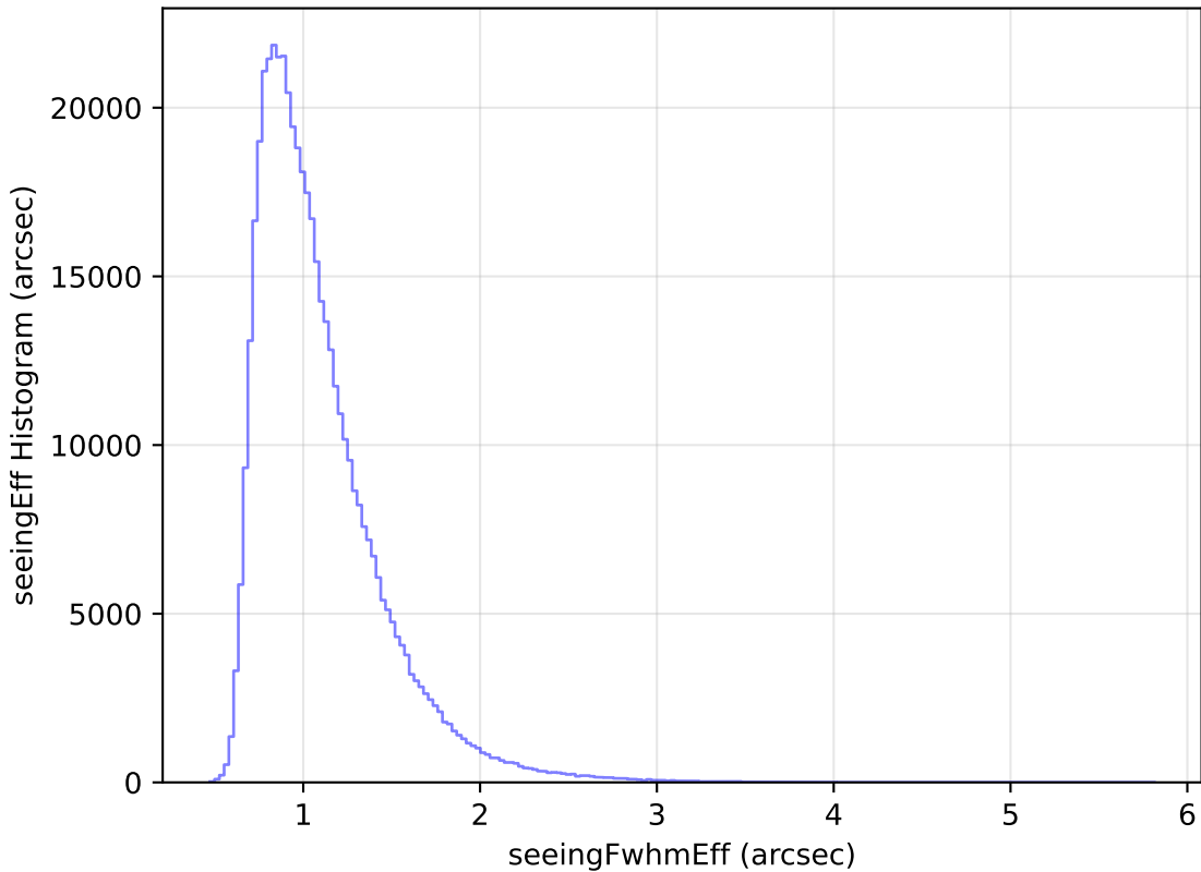
too_elab_r32_d3_ugrizy_v3.4_10yrs WFD i band: seeingEff Histogram
