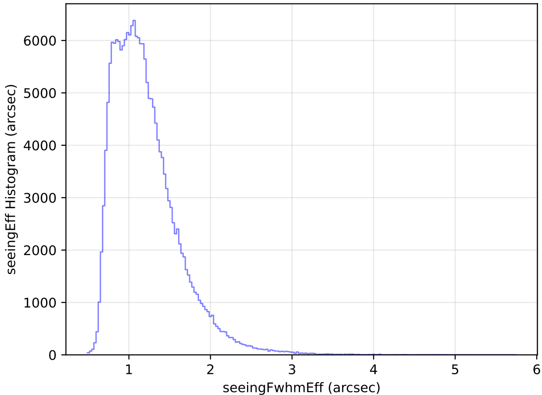
too_elab_r32_d3_ugrizy_v3.4_10yrs WFD g band: seeingEff Histogram
