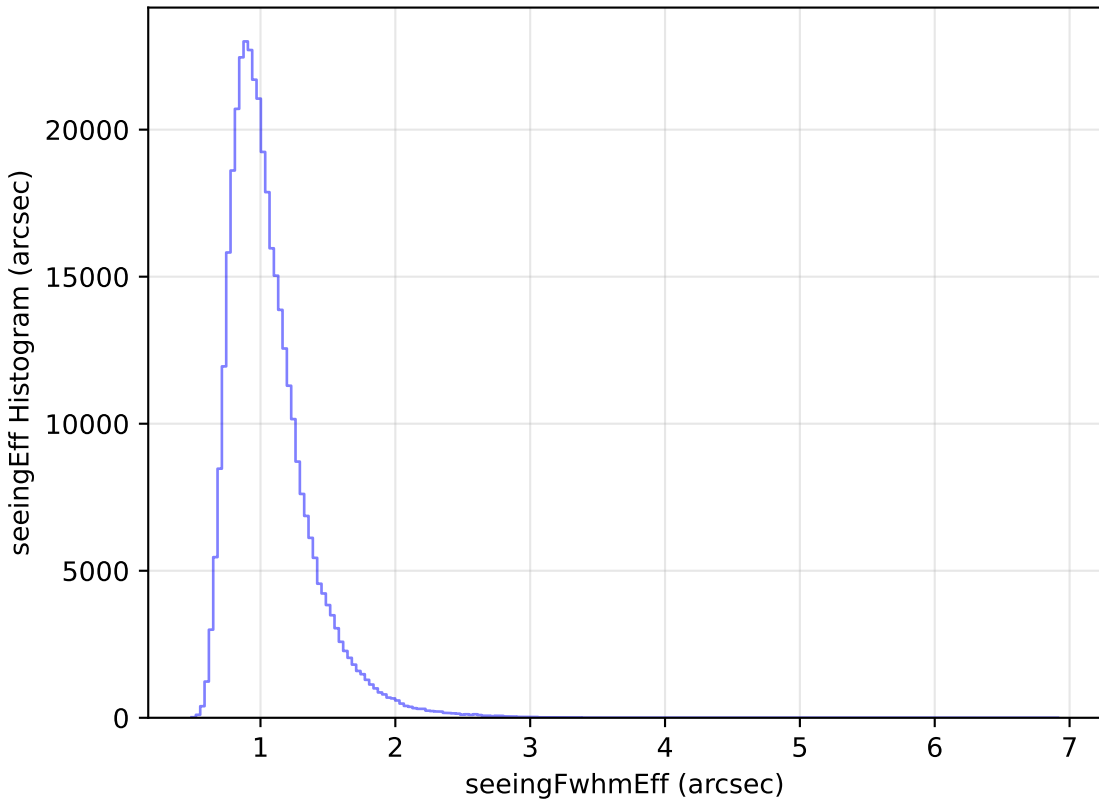
too_elab_r32_d3_ugrizy_v3.4_10yrs All sky y band: seeingEff Histogram
