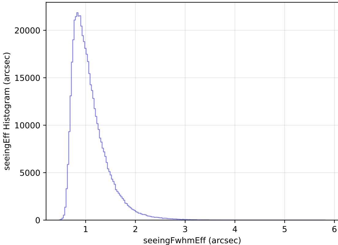
too_elab_r32_d3_ugrizy_v3.4_10yrs All sky i band: seeingEff Histogram
