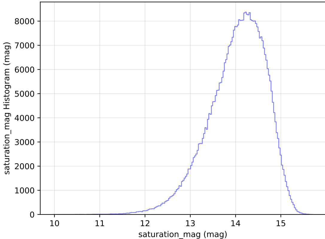
too_elab_r32_d3_ugrizy_v3.4_10yrs WFD z band: saturation_mag Histogram
